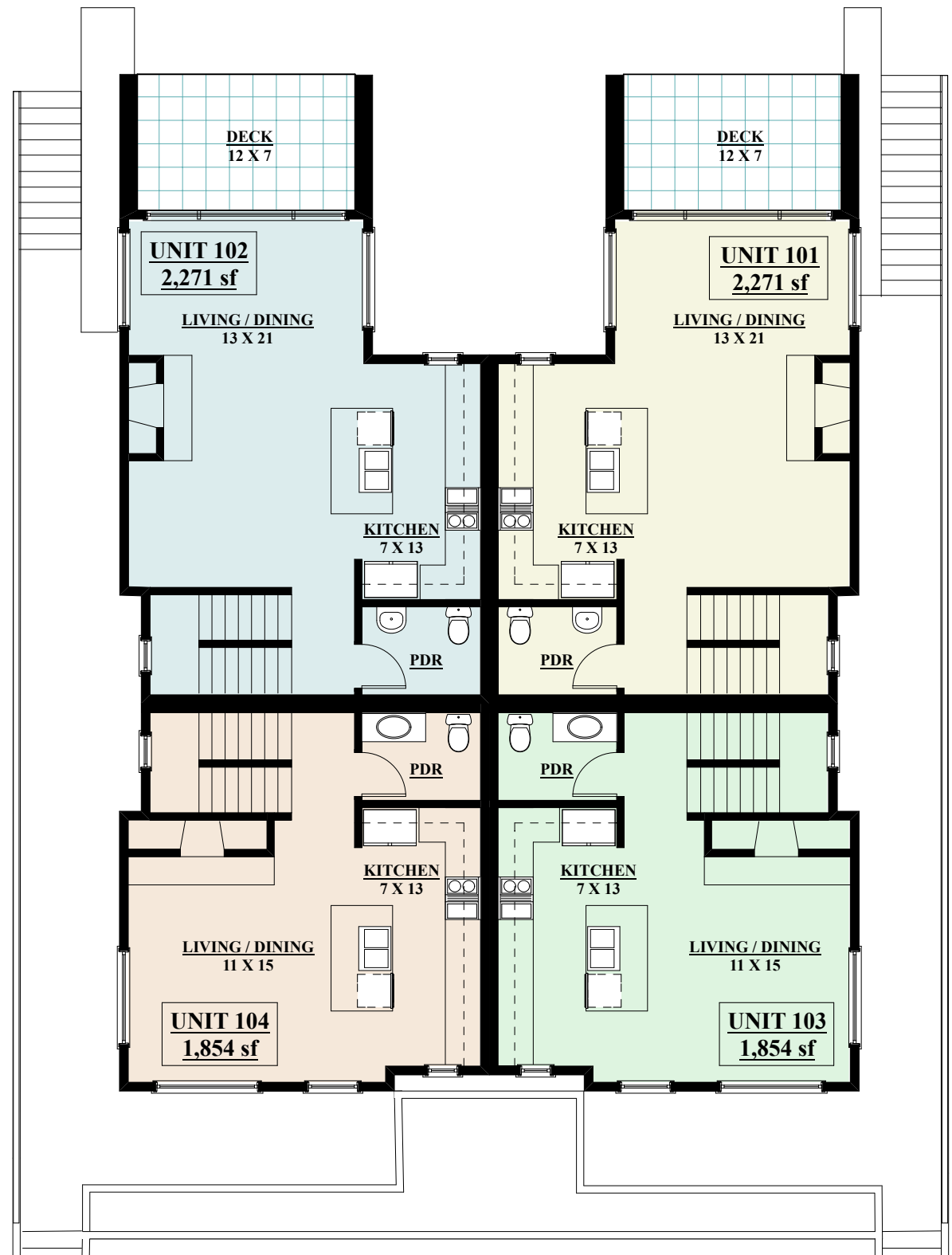
LEVEL 2 PLAN NORTH BUILDING
