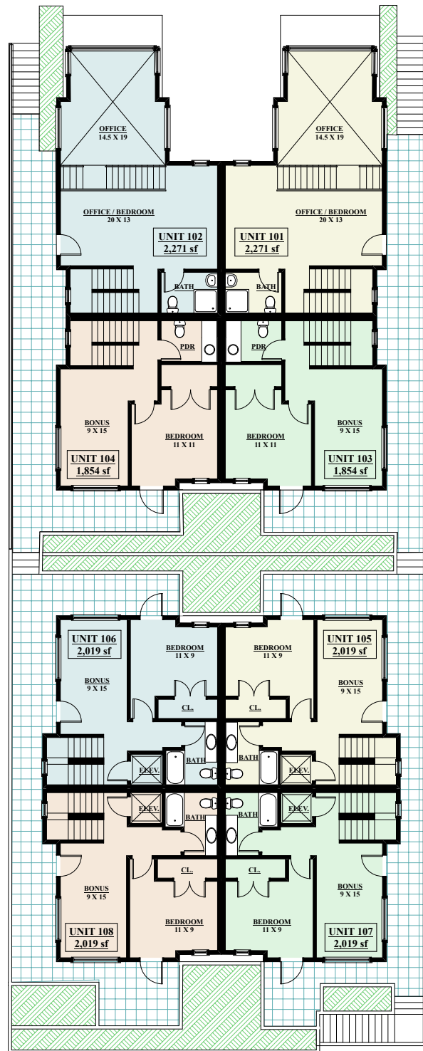
LEVEL 1 PLAN ALL UNITS
